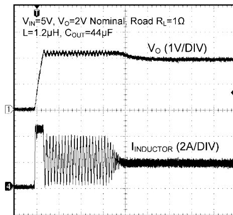
Recovery from Thermal Shutdown - "LMR10530X"
