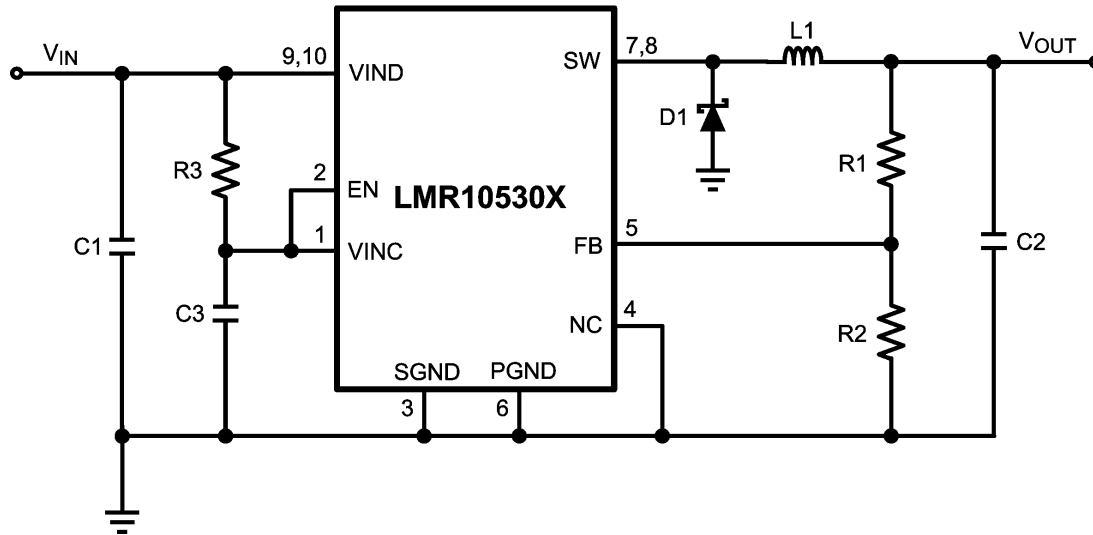
FIGURE 11. LMR10530X (1.5MHz): V_{IN} = 3.3V , Output = 1.2V/3.0A
