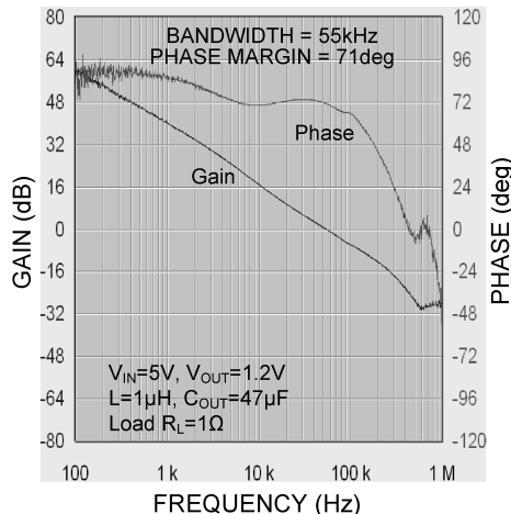
Loop Gain and Phase - "LMR10530Y"
