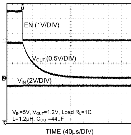
Shutdown by EN - "LMR10530X"
