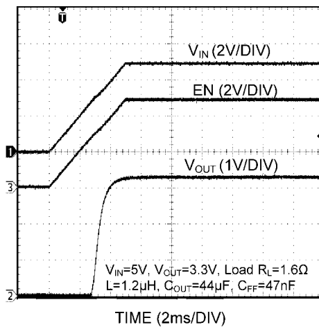
FIGURE 4. Startup Response to V_{IN} with C_{FF}
