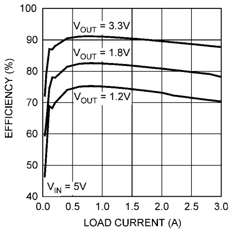
Efficiency vs Load Current - "LMR10530Y"
