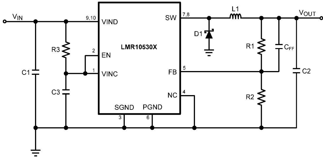
FIGURE 12. LMR10530X (1.5MHz): V_{IN} = 5V , Output = 3.3V/3.0A
