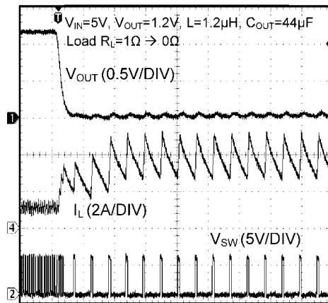
Short-circuit Triggering - "LMR10530X"
