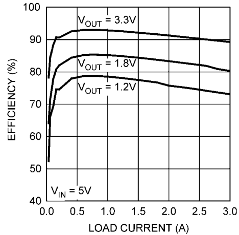
Efficiency vs Load Current - "LMR10530X"
