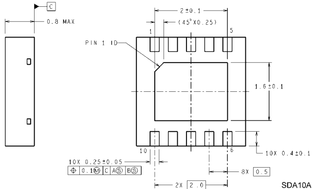
10-Lead LLP Package Package Number SDA10A
