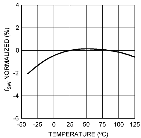
Oscillator Frequency vs Temperature - "LMR10530X"
