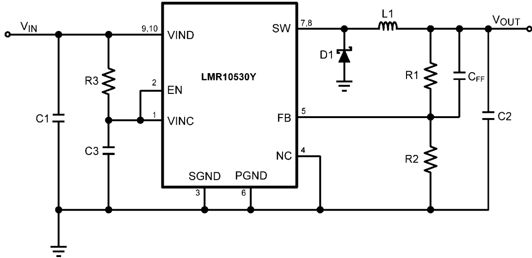
FIGURE 14. LMR10530Y (3MHz): V_{IN} = 5V , Output = 3.3V/3.0A
