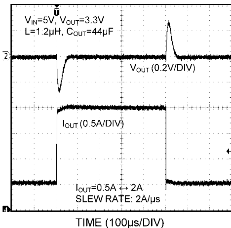
Load Step Response - "LMR10530X"
