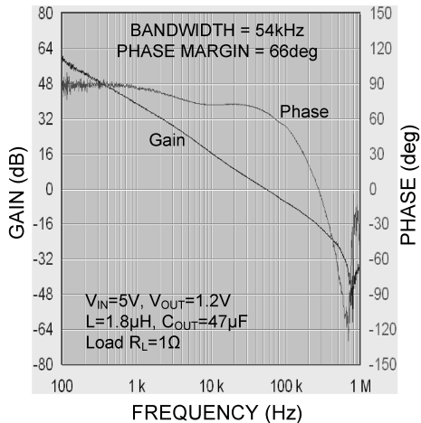
Loop Gain and Phase - "LMR10530X"
