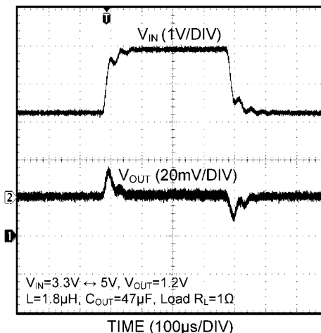
Line Transient Response - "LMR10530X"
