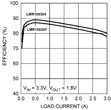
Efficiency vs Load Current - "LMR10530X" and "LMR10530Y"
