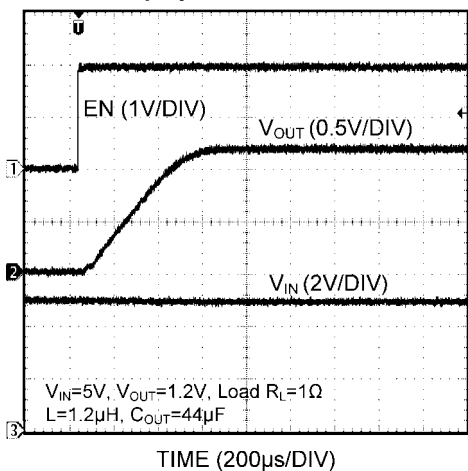
Startup by EN - "LMR10530X"
