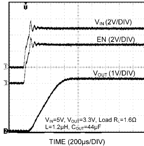
FIGURE 5. Startup Response to V_{IN} with 100µs rise time
