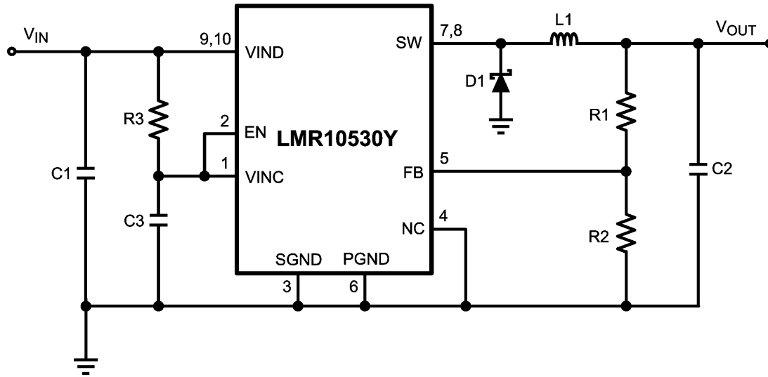
FIGURE 13. LMR10530Y (3MHz): V_{IN} = 3.3V , Output = 1.2V/3.0A
