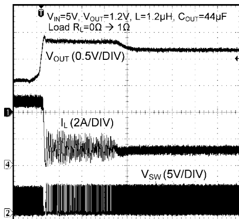
Short-circuit Release - "LMR10530X"
