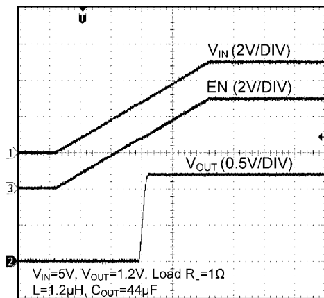
Startup with EN tied to V_{IN} - "LMR10530X"
