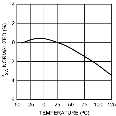
Oscillator Frequency vs Temperature - "LMR10530Y"
